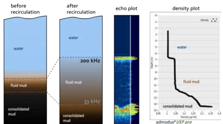
Fluid mud layer before and after recirculation.
